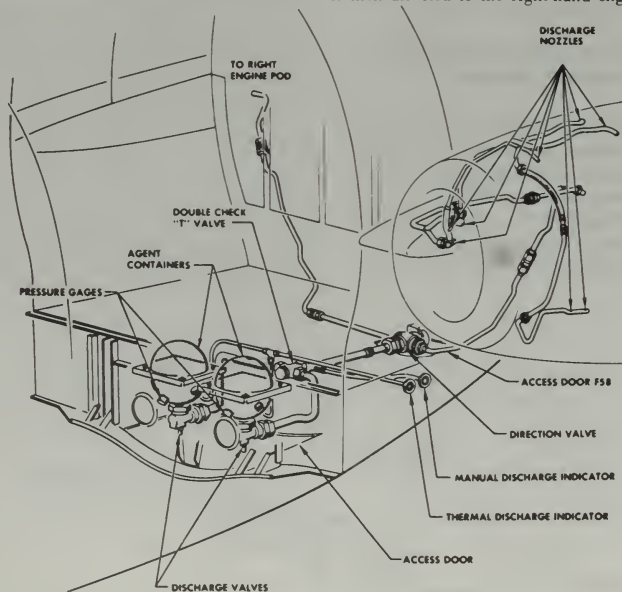
FIGURE 9-24. Fire extinguishing system.
